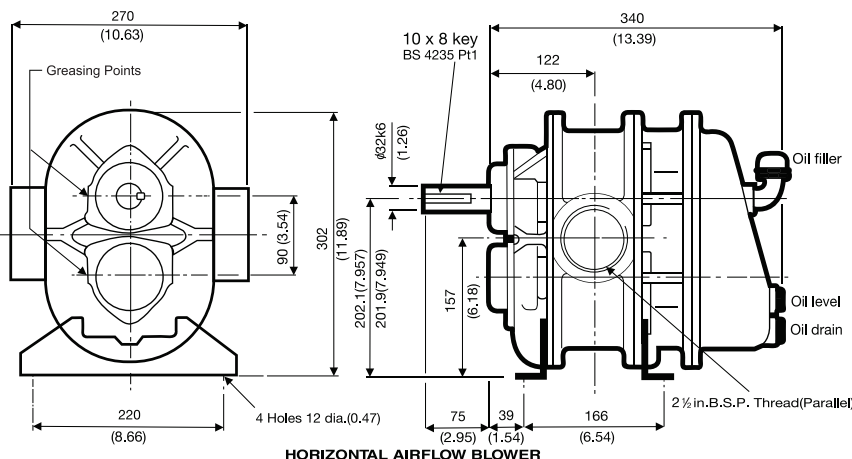
HORIZONTAL AIRFLOW BLOWER
