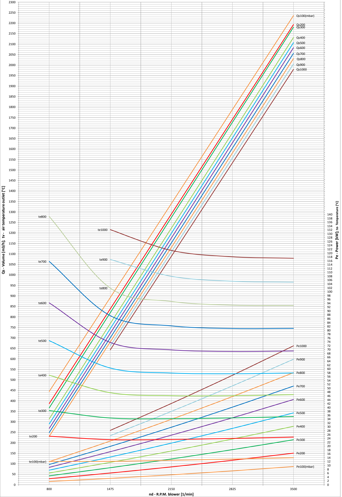
KTSR150 -Volume Flow Rate, Power and Air Temperature in Outlet Vs R.P.M for Pressure Difference 100 - 1000 mbar
