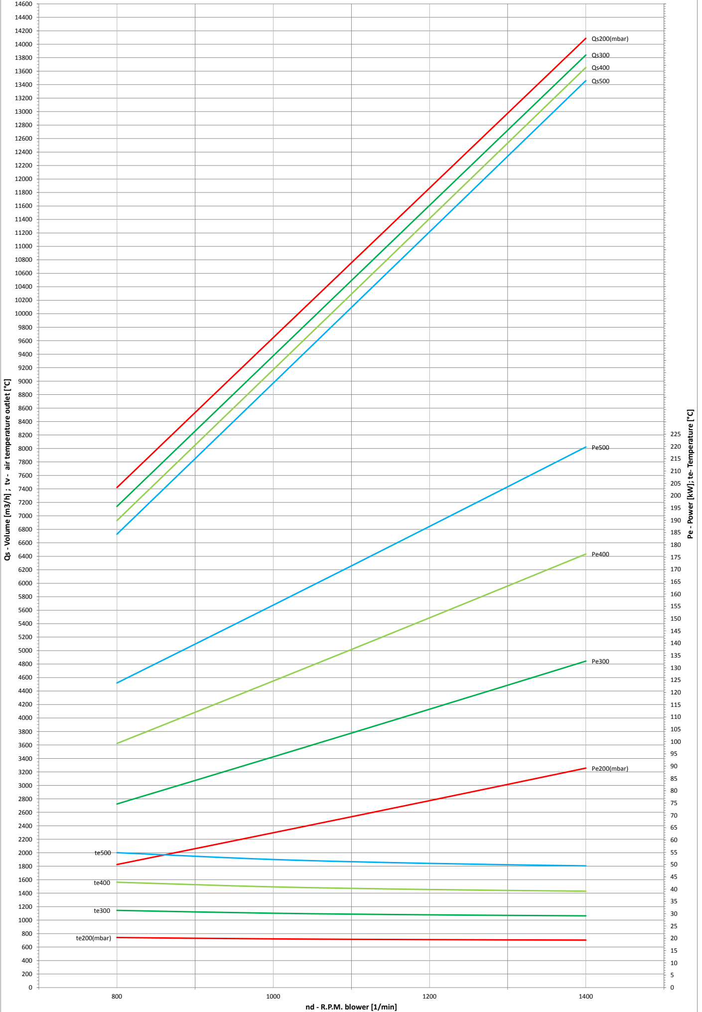
SR1000 -Volume Flow Rate, Power and Air Temperature in Outlet Vs R.P.M for Pressure Difference 200 - 500 mbar
